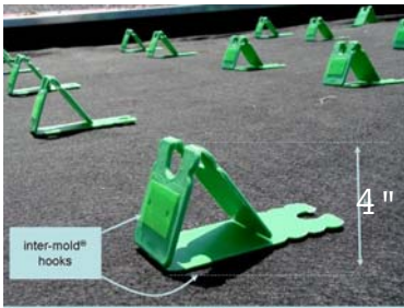
inter-mold® hooks on 2 sides => 2 different heights of the system (H) inter-mold® hooks attach to felt
